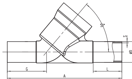
Body size-Welded (mm)
