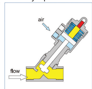
Normally Open Valve
