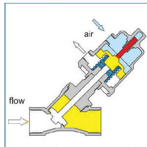
Valve Closed
