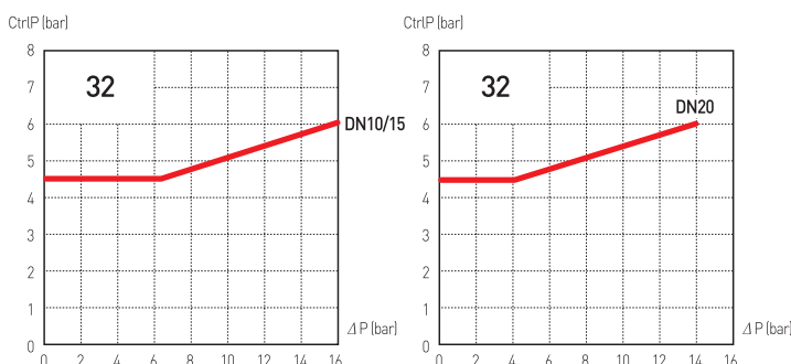
Normally Closed Valve
