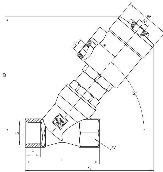
Normally Open
