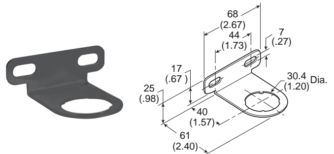
Angle Bracket (Fits to regulator and filter/regulator body) P31KB00MR
