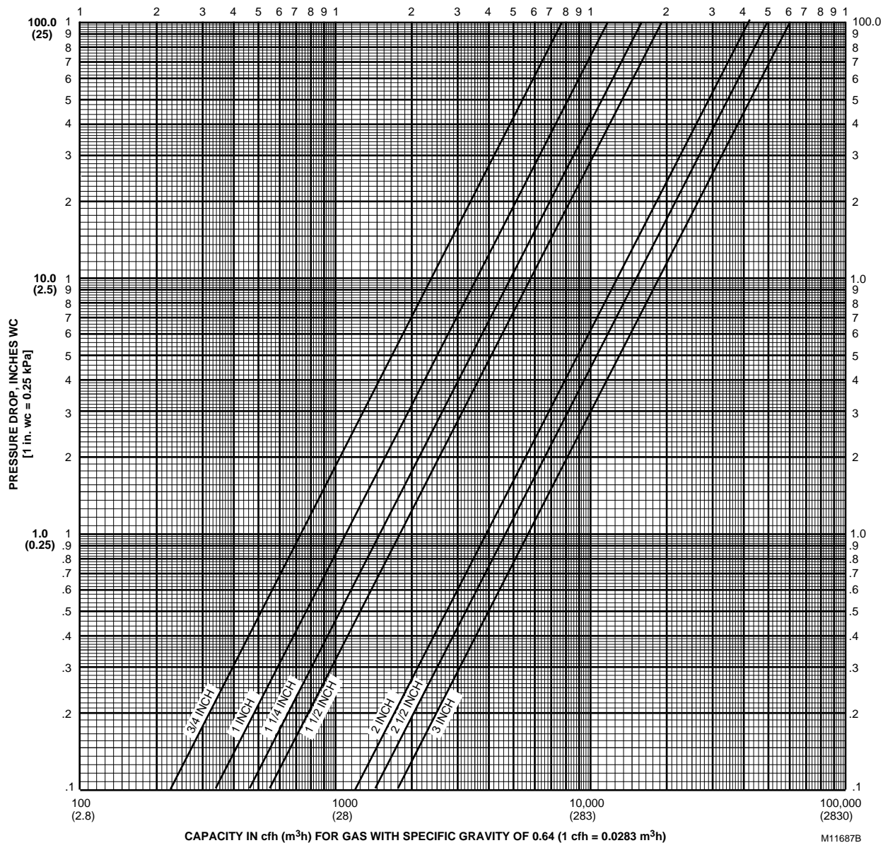
Fig. 3. Flow curves for V5097 Valves.
