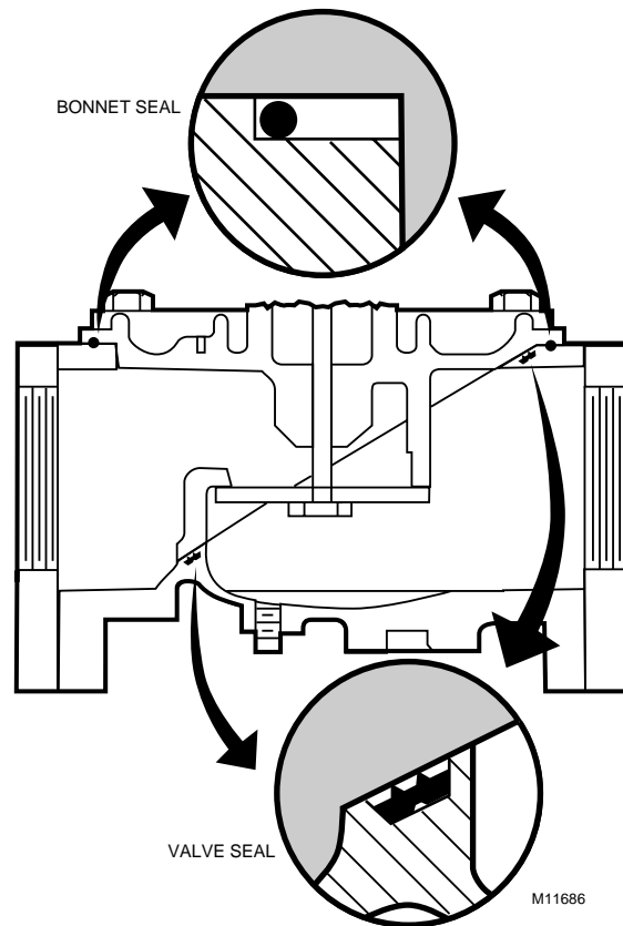
Fig. 5. Proper positions of valve and bonnet seals in V5097 Valves.
